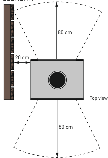
A COMBUSTION CHAMBER WITHOUT LATERAL EXTENSION ELEMENT:
